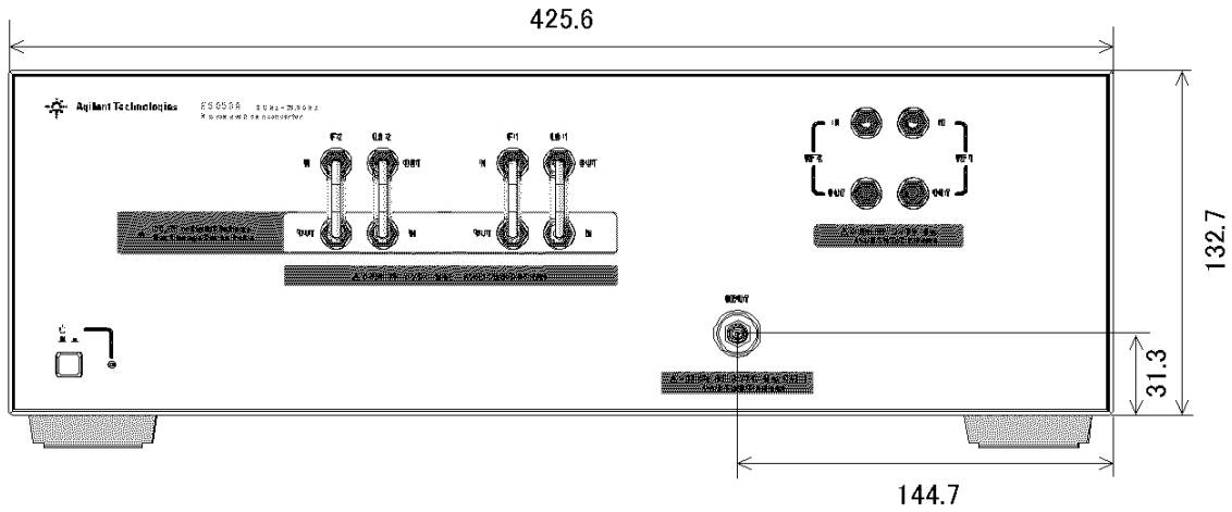
Figure 10-6. Front view
